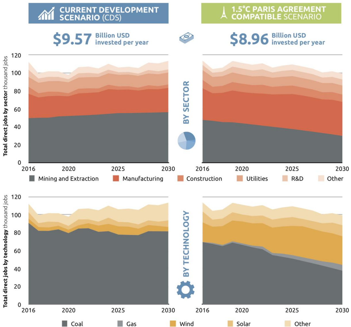
Figure 15: 'Total direct jobs per employment sector' and 'Total direct jobs per generation technology' between 2016-2030 for the Current Development Scenario (CDS) (graphs on left) and the 1.5°C Paris Agreement compatible scenario for the South African electricity supply sector (graphs on right). Direct employment estimates reflect energy supply sector investments linked to planning, construction, the manufacturing of component parts, operation (including fuel supply such as coal mining, where relevant) and maintenance of power plants.
